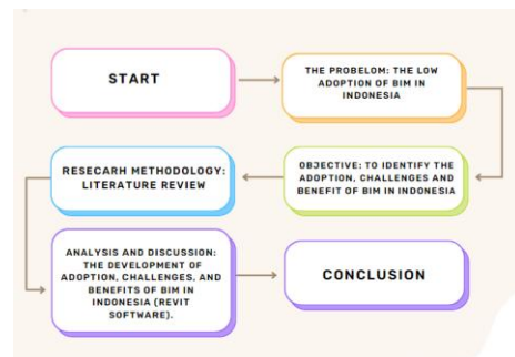
Figure 3. FlowChart
