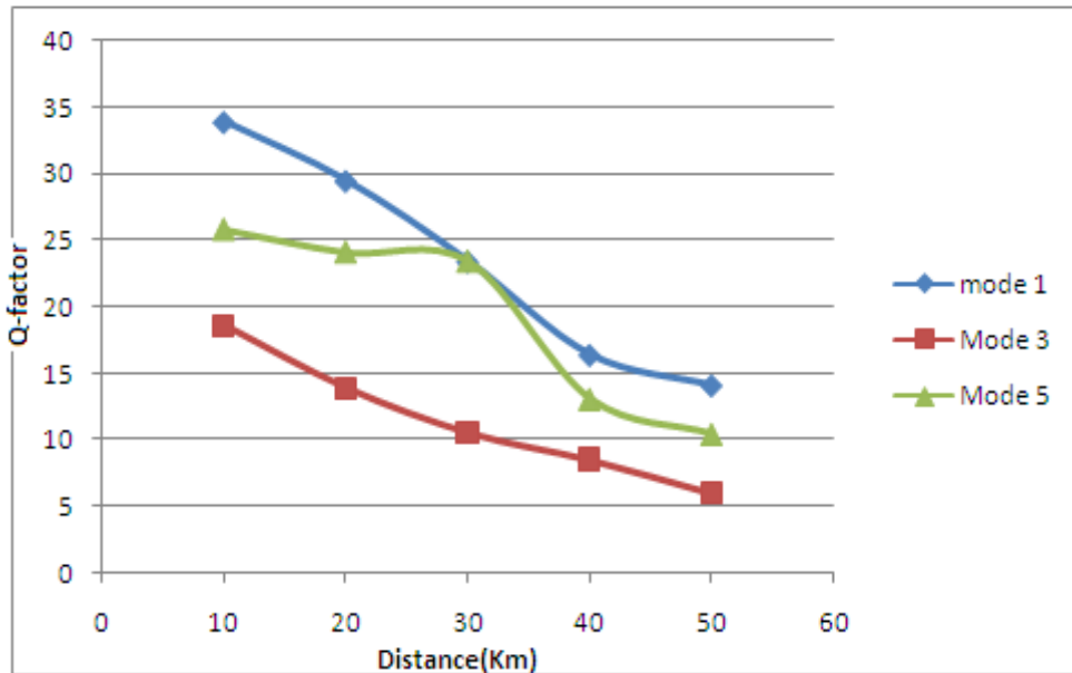
Fig 6 Graphical representation of 0mode 1,2 and 3 vs distance
