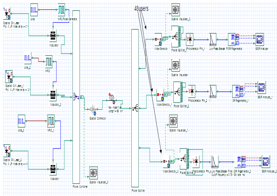
Fig 1 System setup for mode multiplexed PON
