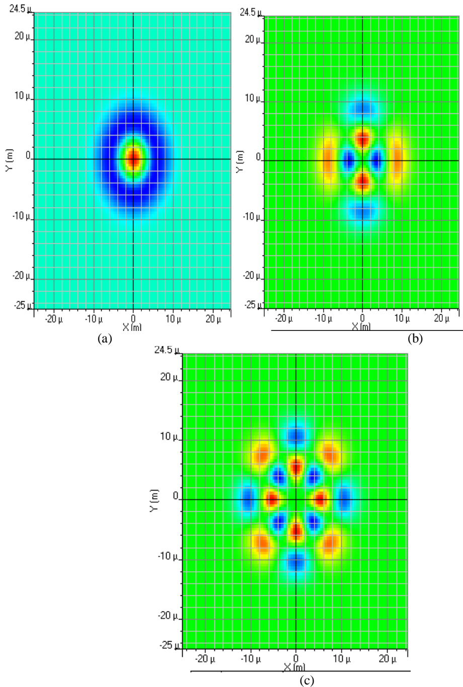
Fig 3 Linearly mode profiles for (a) Mode 1 (b) Mode 3 (c) Mode 5
